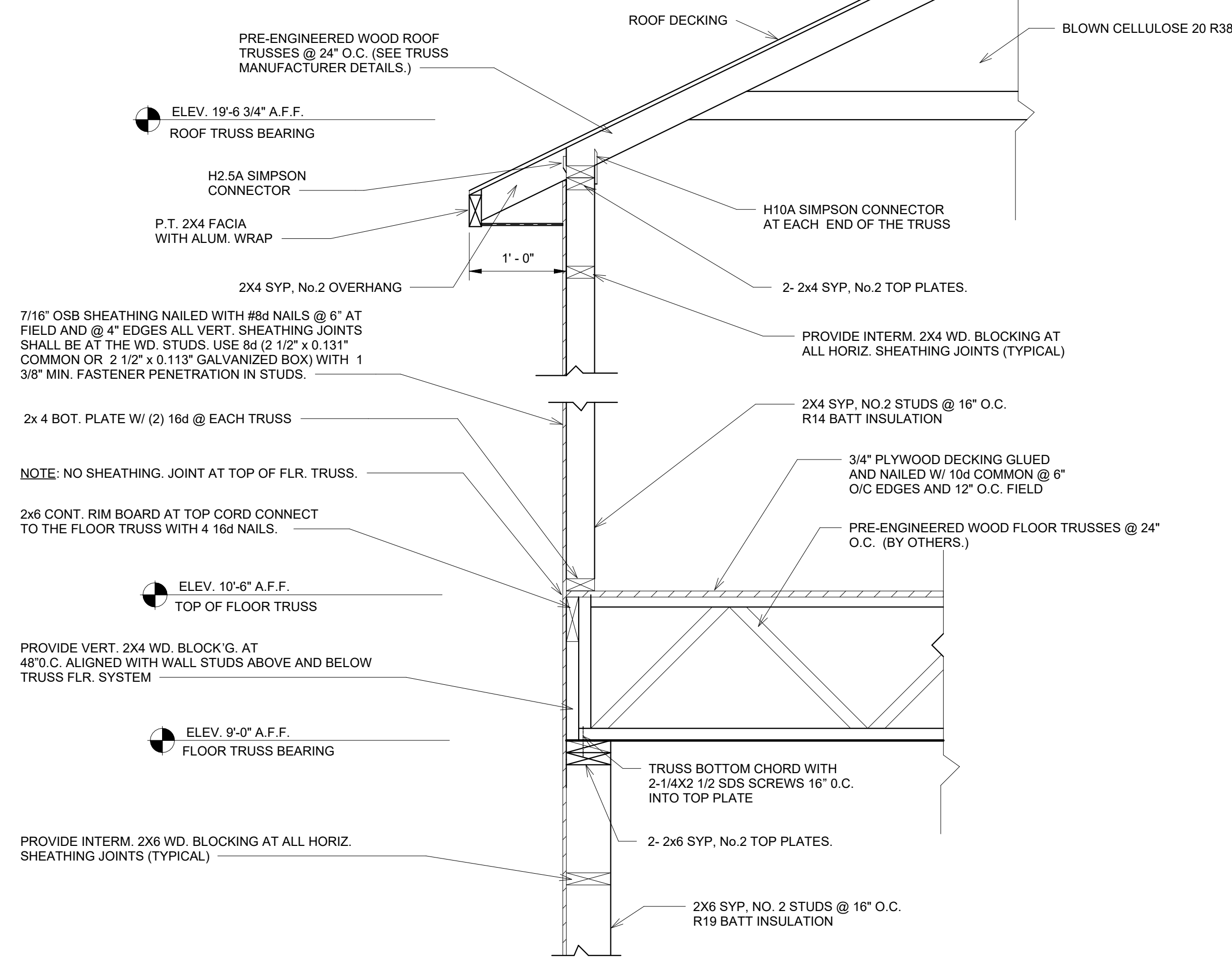
5 EXTERIOR WALL SECTION_2 1" = 1'-0"
