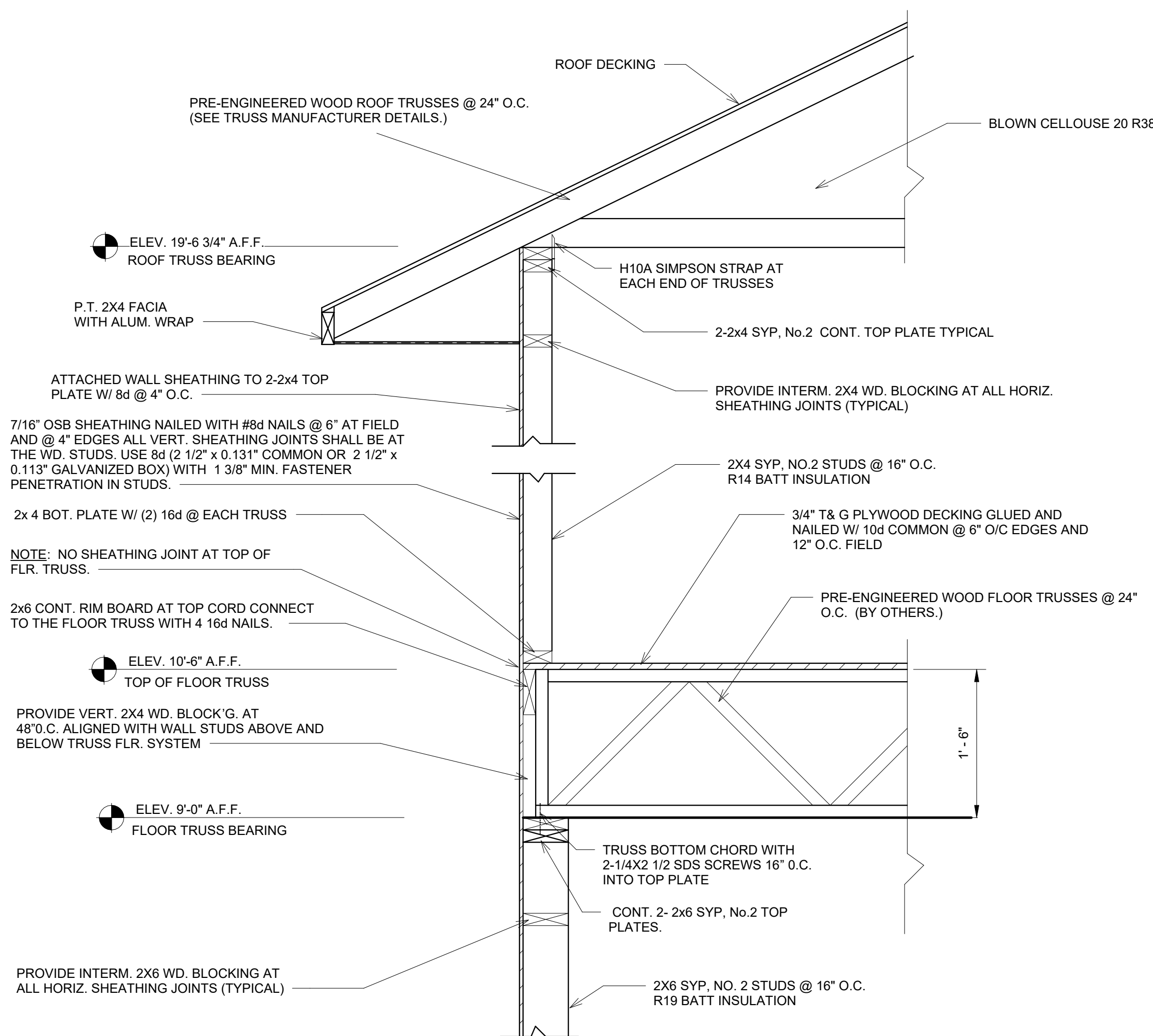
6 EXTERIOR WALL SECTION_1 1" = 1'-0"
