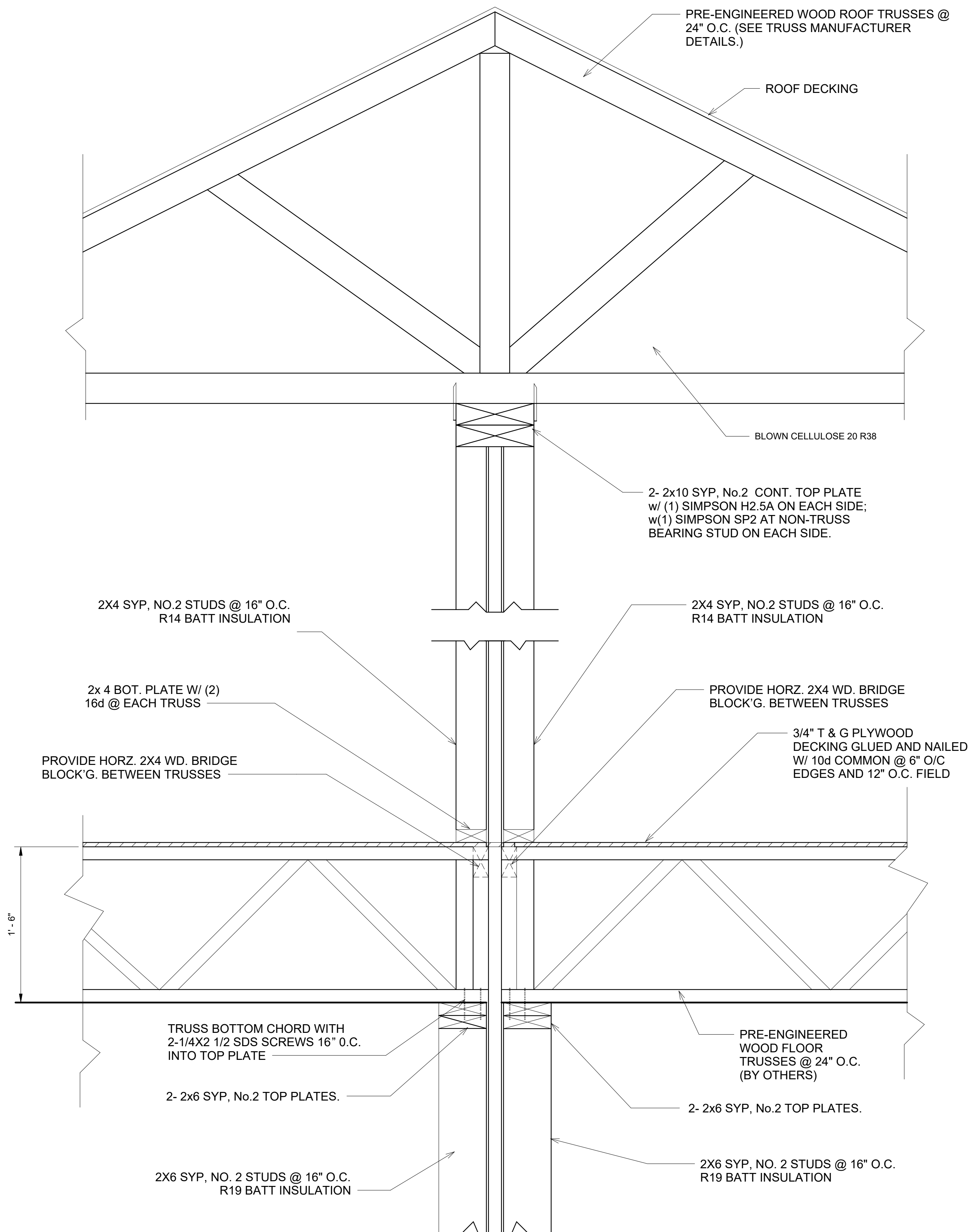
1 INTERIOR WALL SECTION 1 1/2" = 1'-0"
